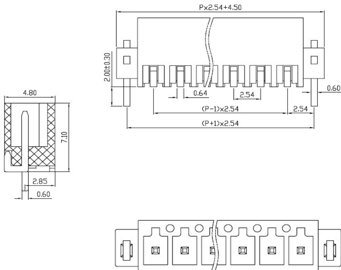
Drawing (Dimension in mm)
