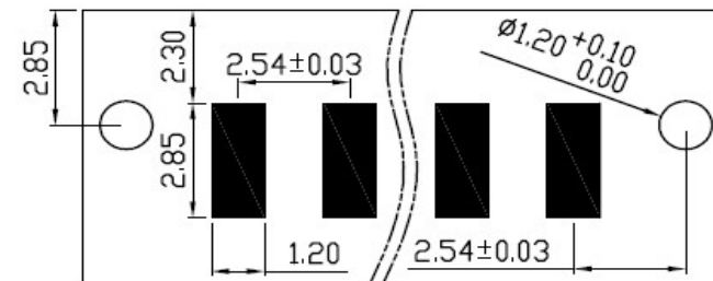
PCB Layout (mm)
