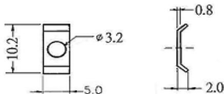
WASHER x4pcs
