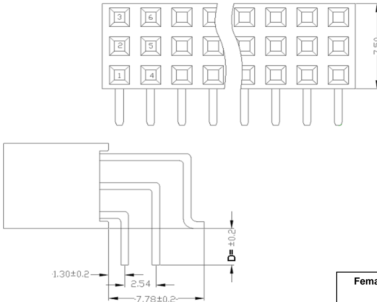
Drawing (mm)
