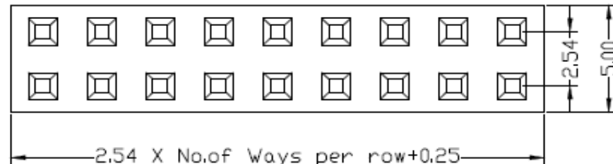
Drawing (mm)
