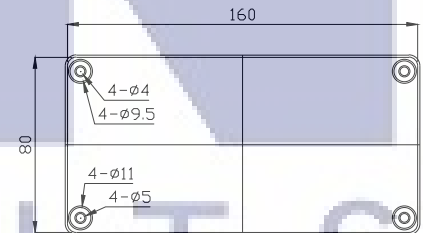
COVER-TOP
