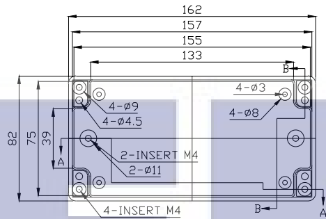
BODY-TOP
