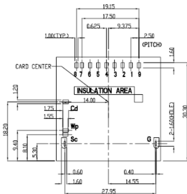
PCB Layout
