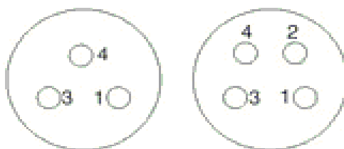
Pin Assignment
