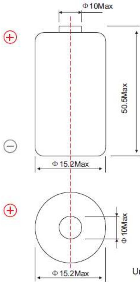
Dimensions (mm)
