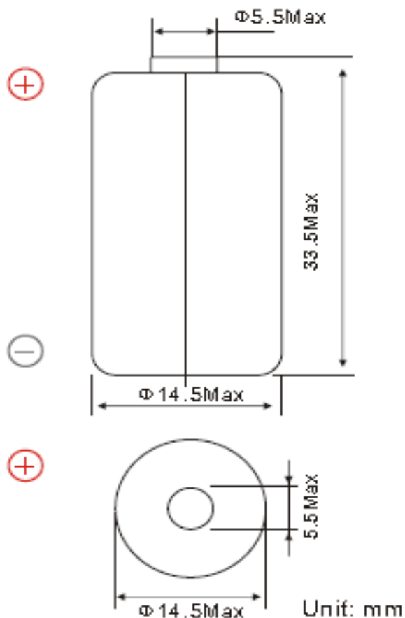
Dimensions (mm)
