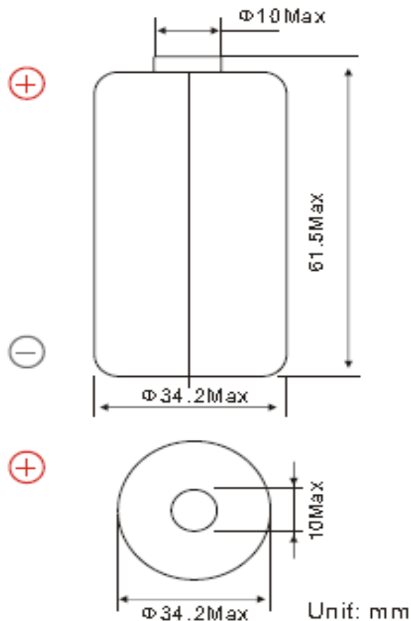
Dimensions (mm)
