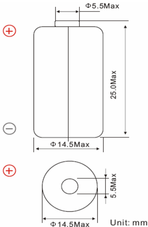
Dimensions (mm)
