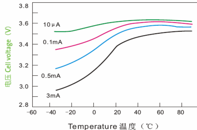
Voltage vs temperature curve
