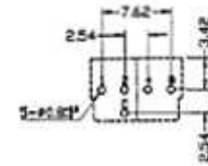
PCB Layout (mm)
