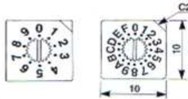
Technical Dimensions (mm)
