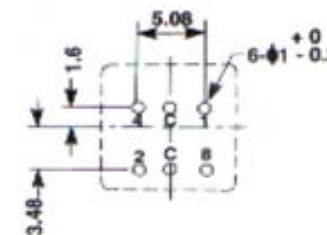
PCB Layout (mm)
