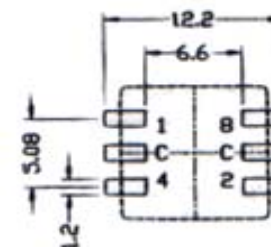
PCB Layout (mm)
