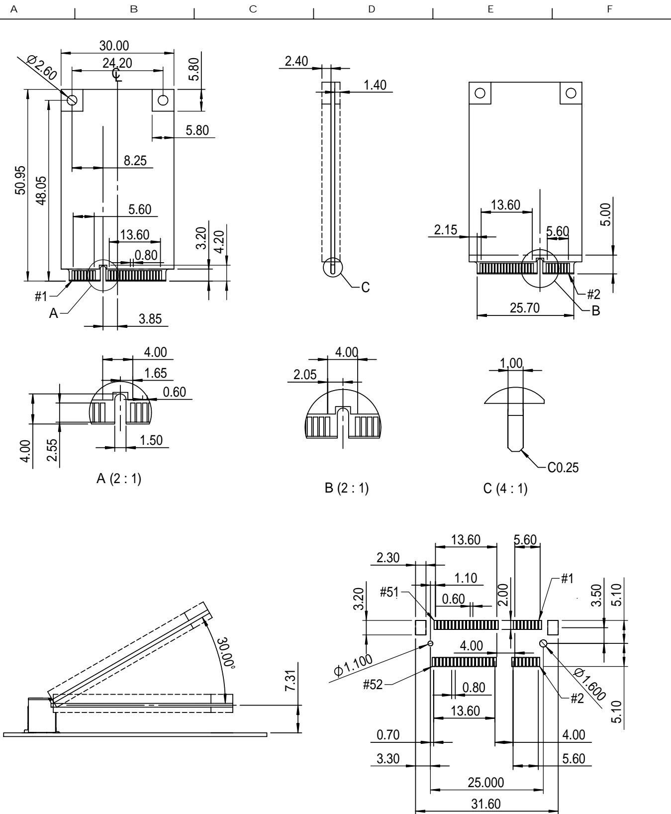
PCB LAYOUT
