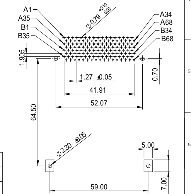
PCB LAYOUT : COMPONENT SIDE
