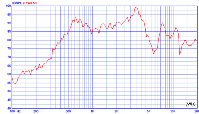
Tested by LMS at 1W 0.5m
