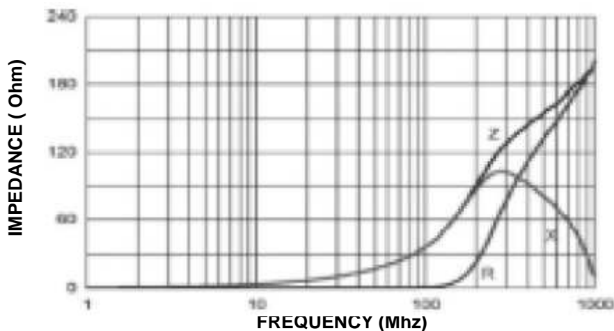
Typical Impedance v.s. Frequency Curve:
