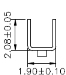
SEC:C-C
