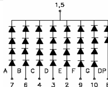
Diode Drive Code B
