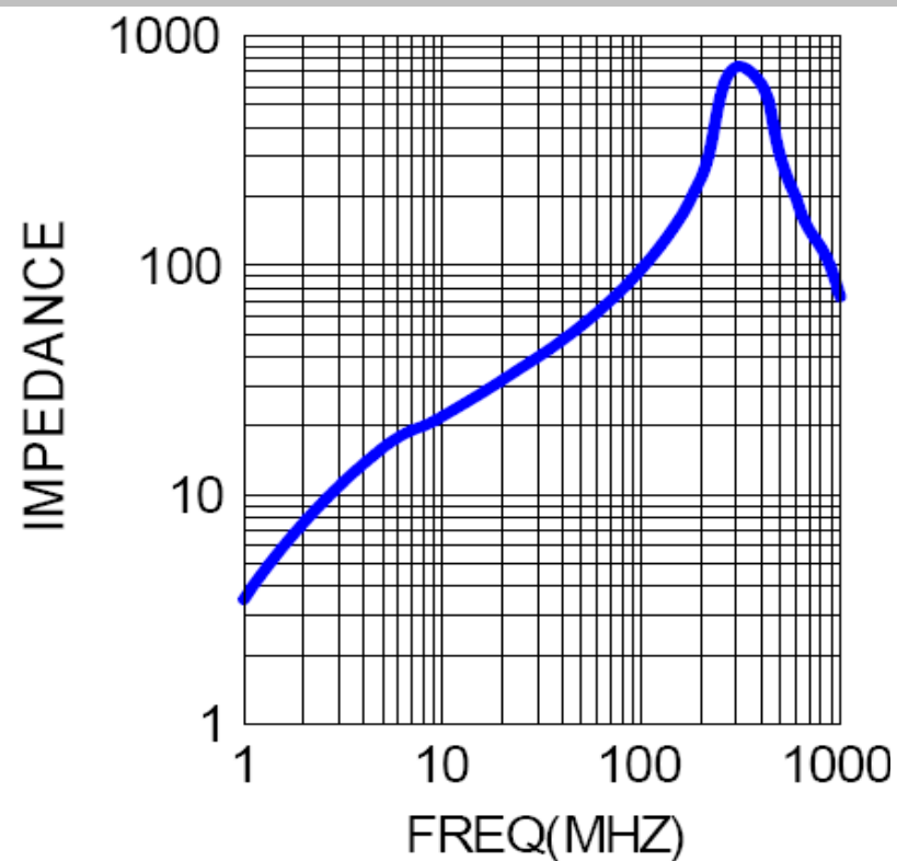
Material K5B
