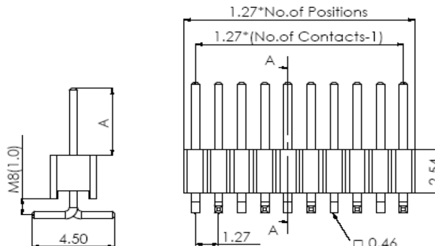
A TYPE
