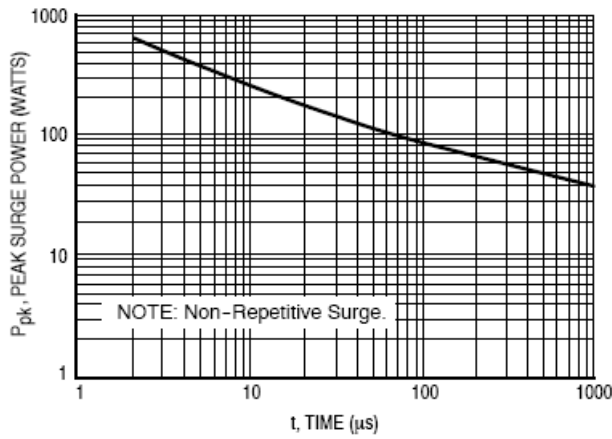
Figure 1. Pulse Width
