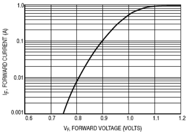
Figure 5. Forward Voltage
