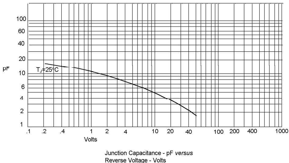
Figure 2 Junction Capacitance
