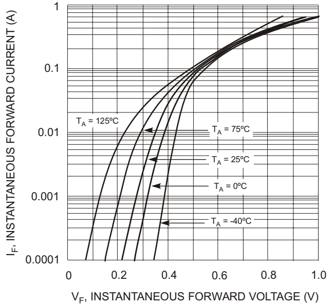
Fig. 2 Forward Characteristics
