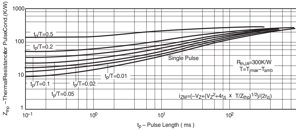
Fig. 10 Thermal Response
