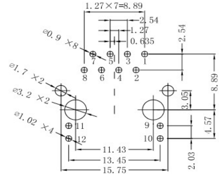
PCB-View Component Side (mm)
