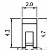
Height f. No of Contacts 4 to 14Pin
