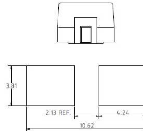
Recommended Pad Layout
