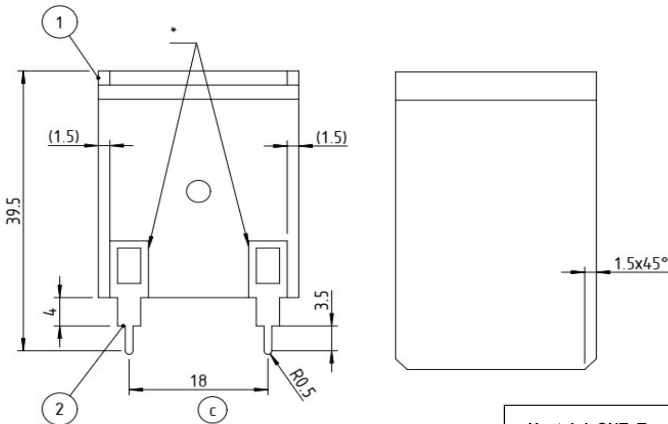
Heatsink SNT Type 2
