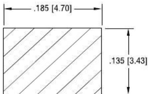
MOUNTING PAD DETAIL
