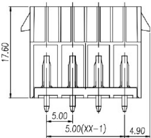
Dimensions / Tolerance (mm)
