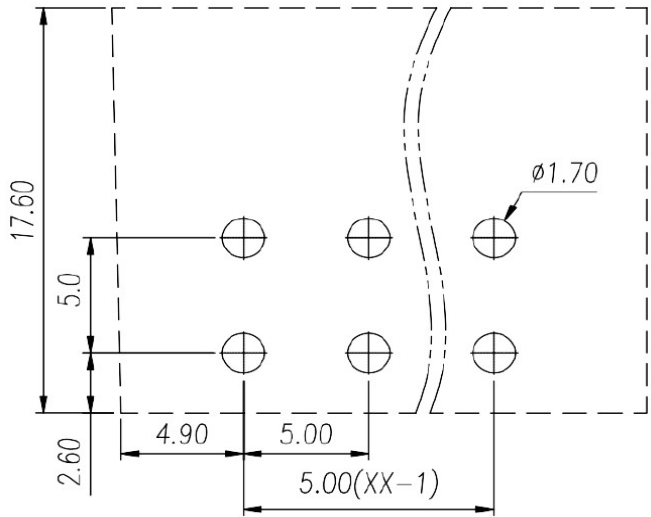
PCB Layout
