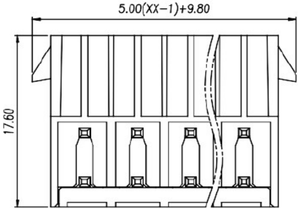
Dimensions / Tolerance (mm)
