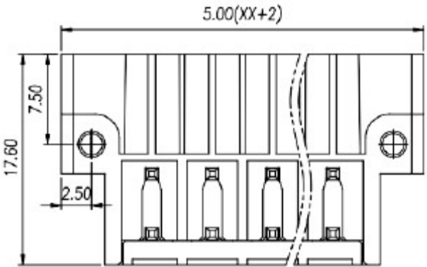
Dimensions / Tolerance (mm)
