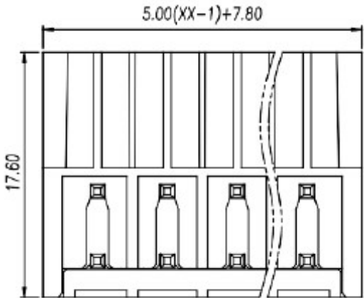
Dimensions / Tolerance (mm)
