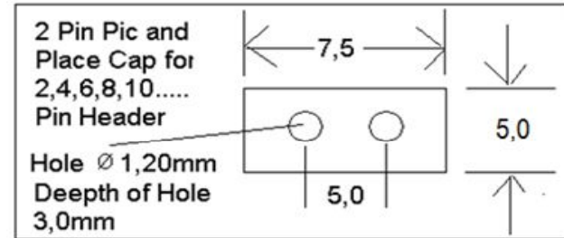
Drawing (Dimension in mm)
