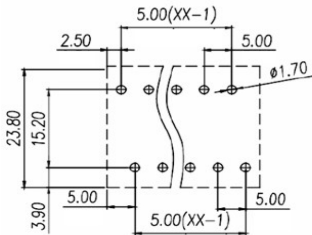
PCB Layout
