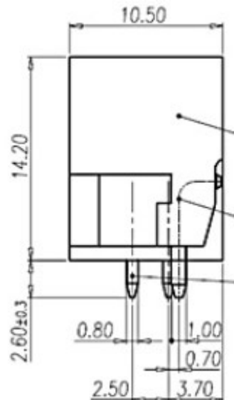
Drawing (Dimension in mm)
