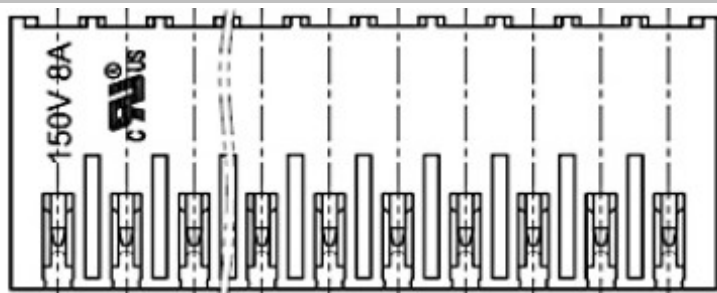
Drawing (Dimension in mm)
