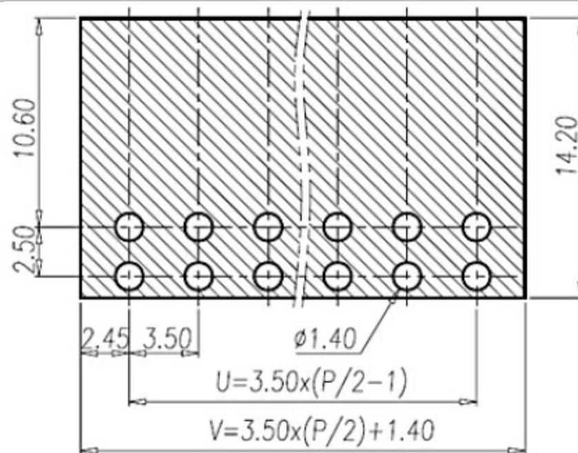
PCB Layout (unit /mm) PCB View
