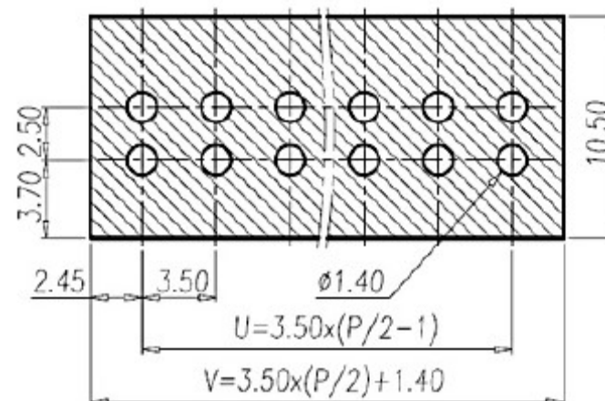
PCB Layout (unit /mm) PCB View
