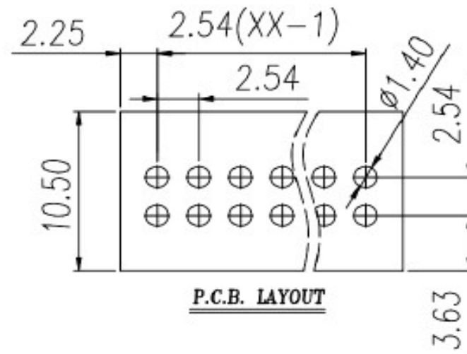
PCB Layout (unit /mm) PCB View
