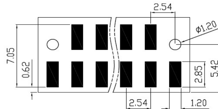
PCB Layout (unit /mm) PCB-View
