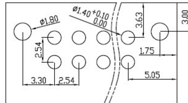
PCB Layout (unit /mm) PCB-View
