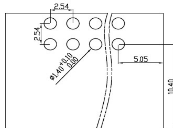
PCB Layout (unit /mm) PCB-View
