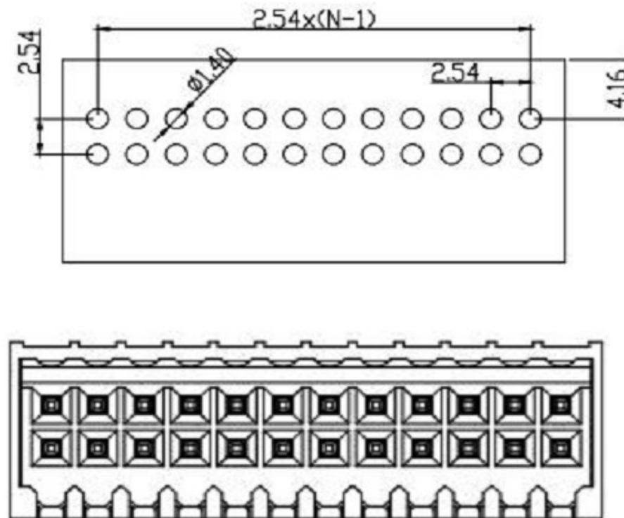
PCB Layout (unit /mm) PCB-View
