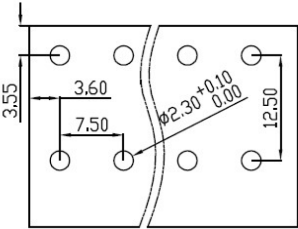
PCB Layout Dimension (mm) TOP-VIEW to PCB
