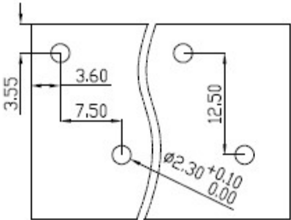
PCB Layout Dimension (mm) TOP-VIEW to PCB
