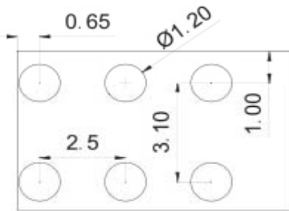
PCB Layout (Dimension in mm)
